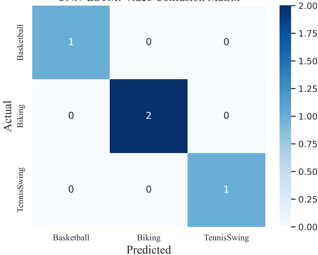
CNN-LSTM: Video Confusion Matrix
